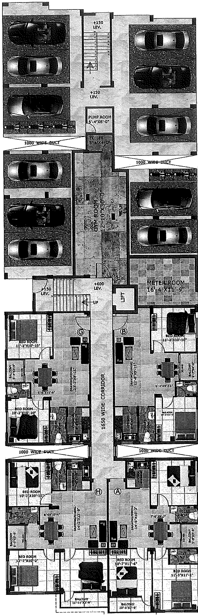
GROUND FLOOR BLOCK-MEGHNA
