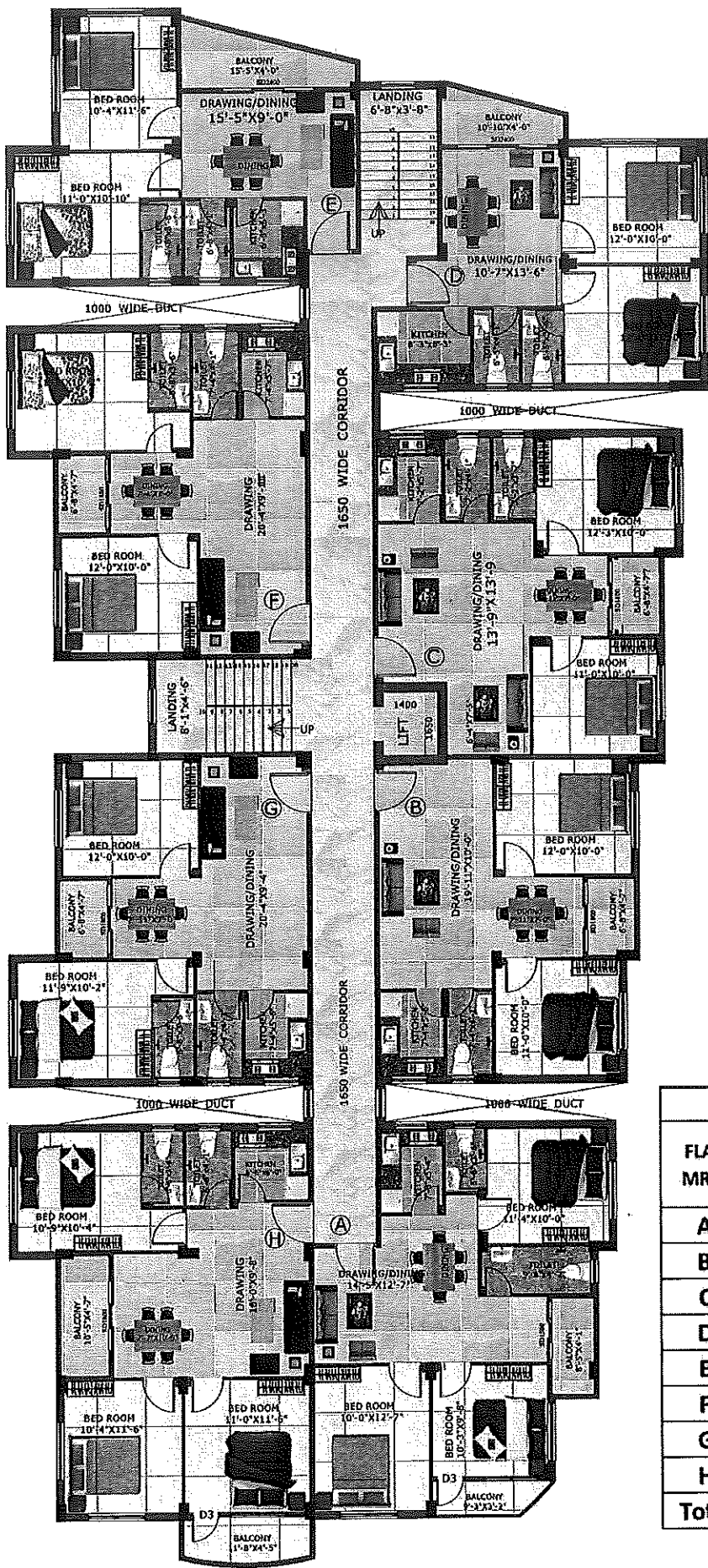
TYPICAL FLOOR PLAN BLOCK- KAVERI
