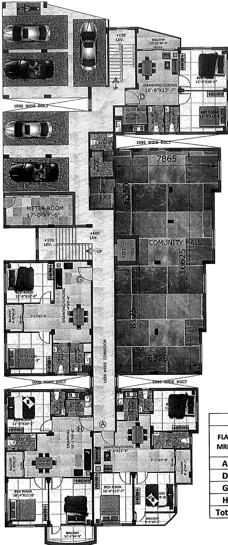
GROUND FLOOR PLAN BLOCK- KAVERI
